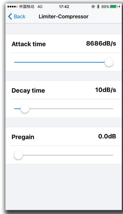
Fig 26. Limiter-Compressor window.
