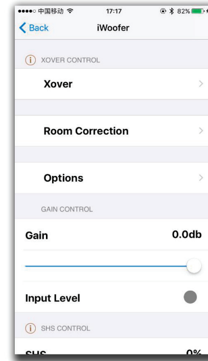
Fig 24. Main window.
