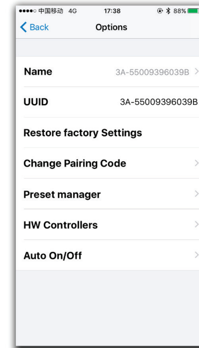
Fig 20. Options window.
