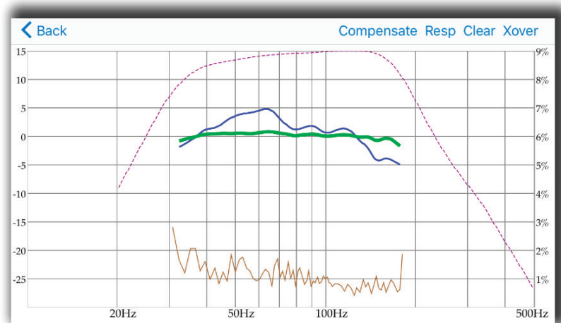
Fig 12. Result response after compensation
